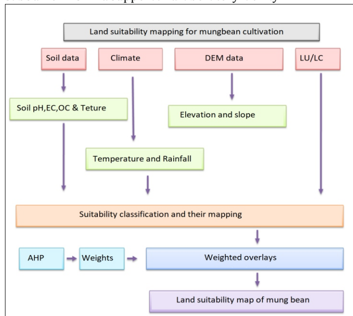
Fig. 2 Flow chart of Land suitability
