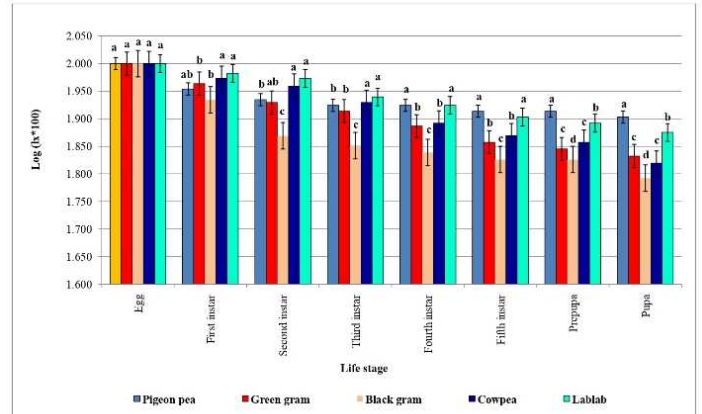
Fig. 2 Survivorship curve of M. vitrata on different pulses under in vitro
