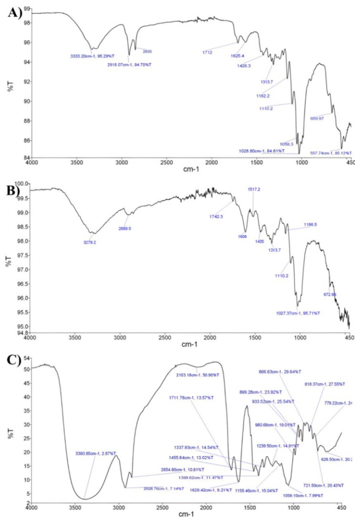
Figure 1: FTIR spectra of (A) 100% B. arundinacea leaf extract, (B) 100% Terminalia arjuna bark extract, and (C) their 90:10 mixture, highlighting key functional groups such as hydroxyl, carbonyl, and C-H stretching, along with the presence of major bioactive compounds, reflecting the complementary properties of both extracts.
